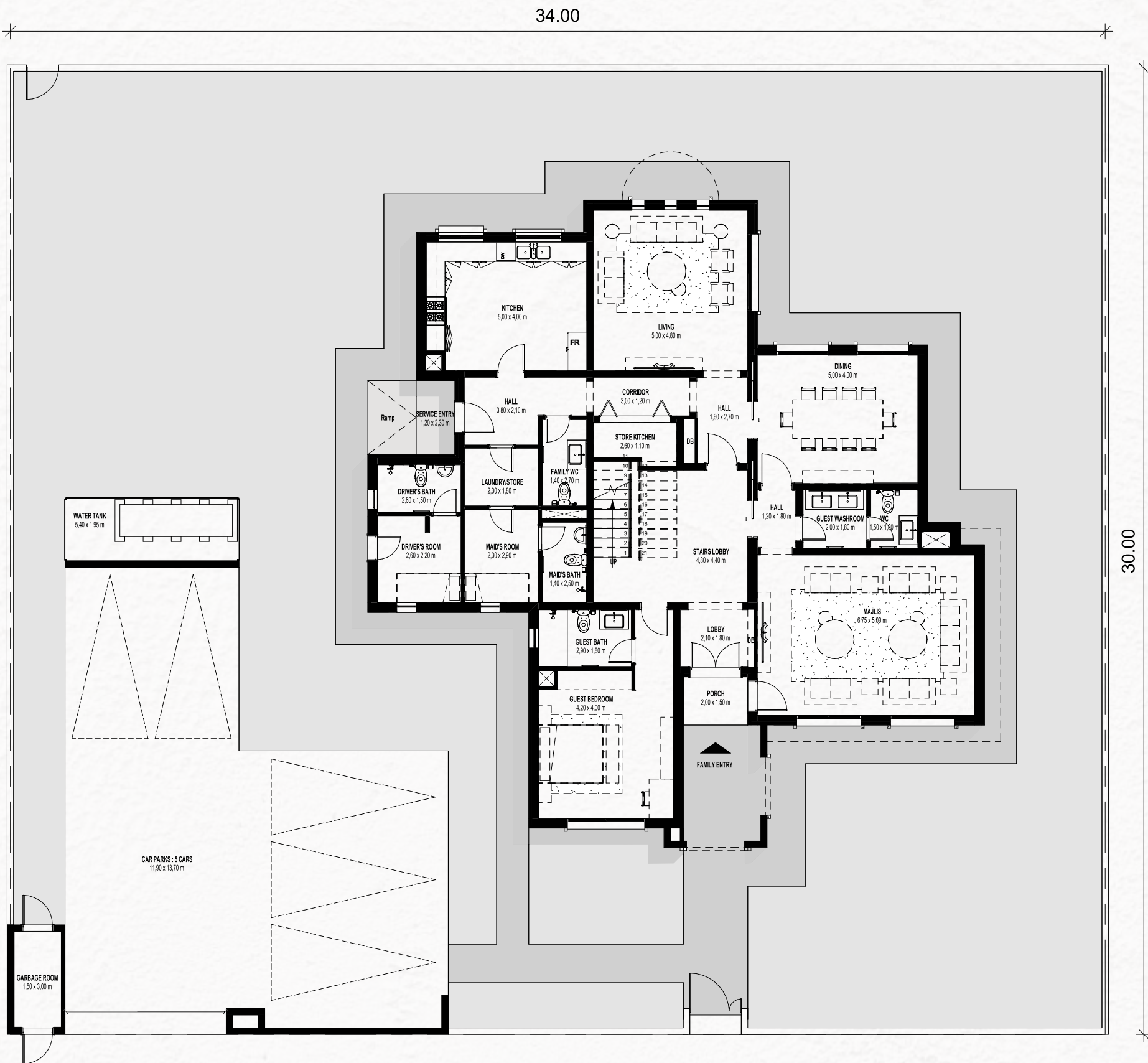
GROUND FLOOR
