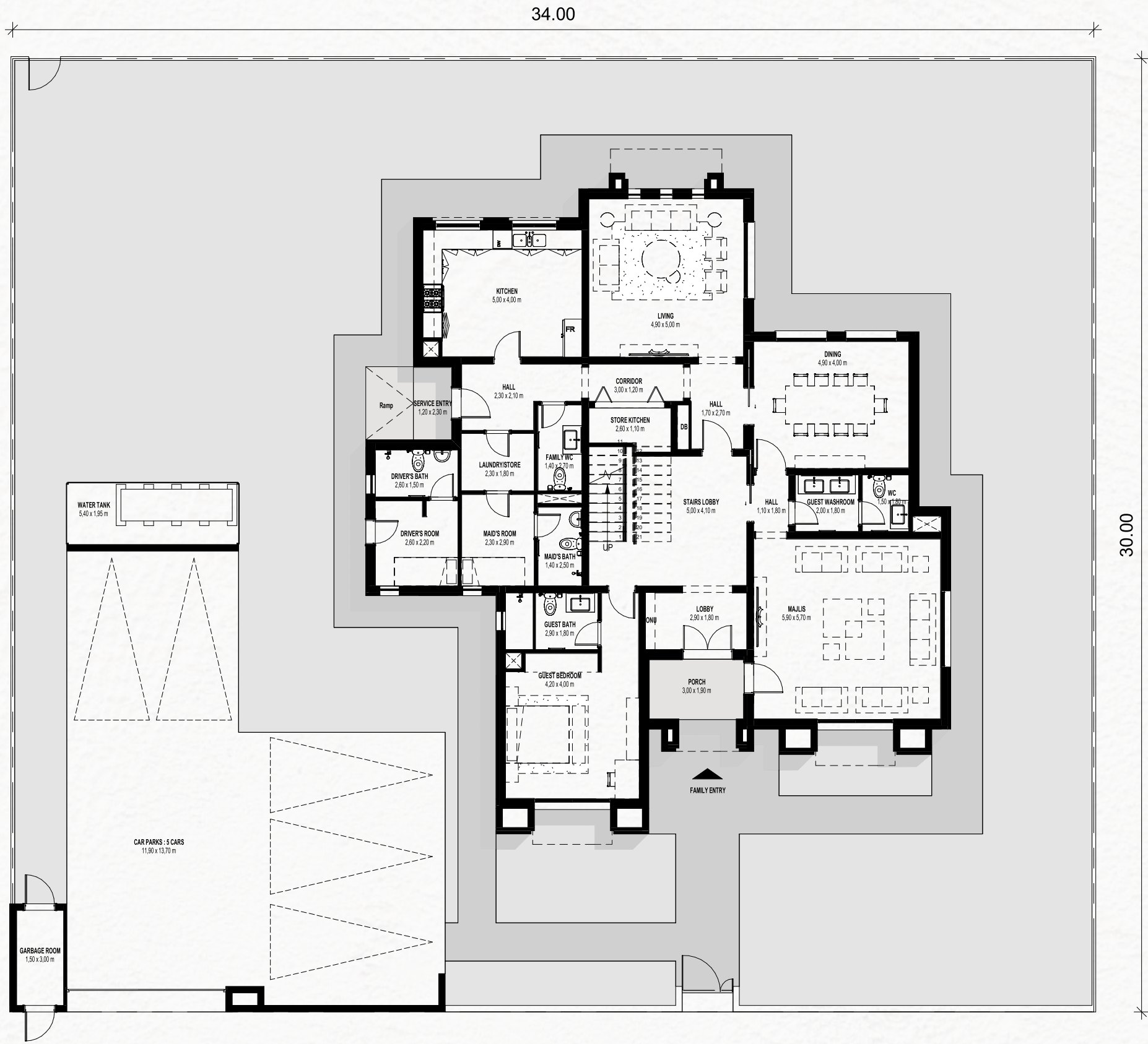
GROUND FLOOR
