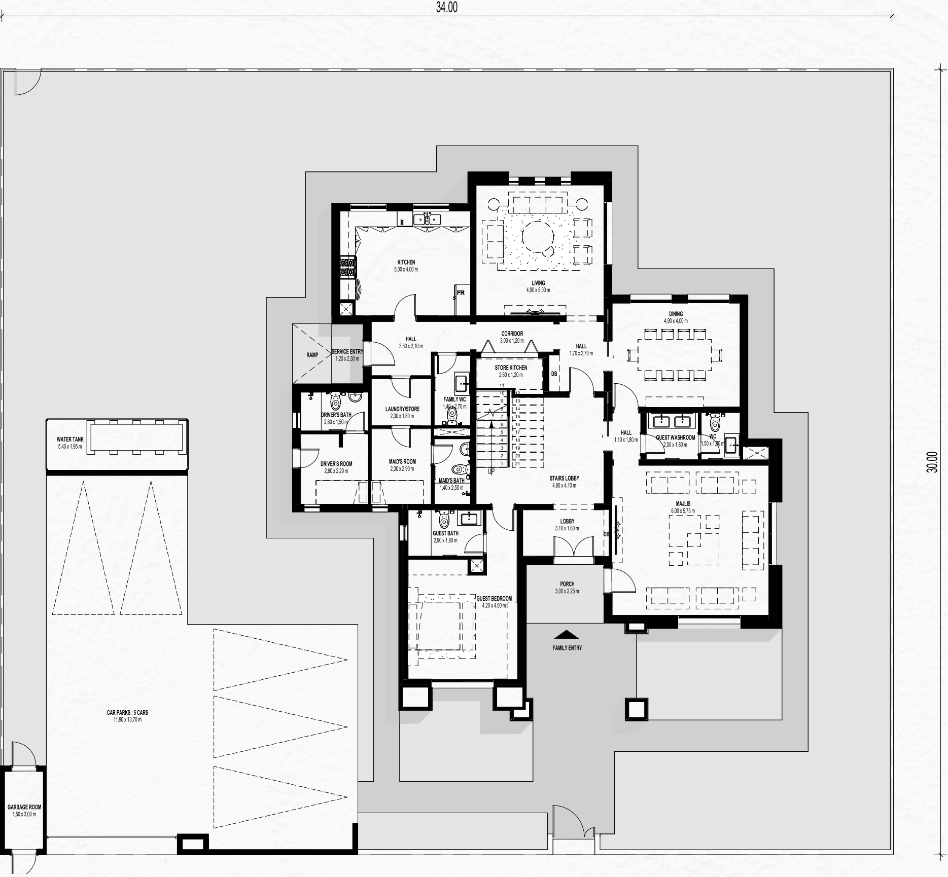
GROUND FLOOR
