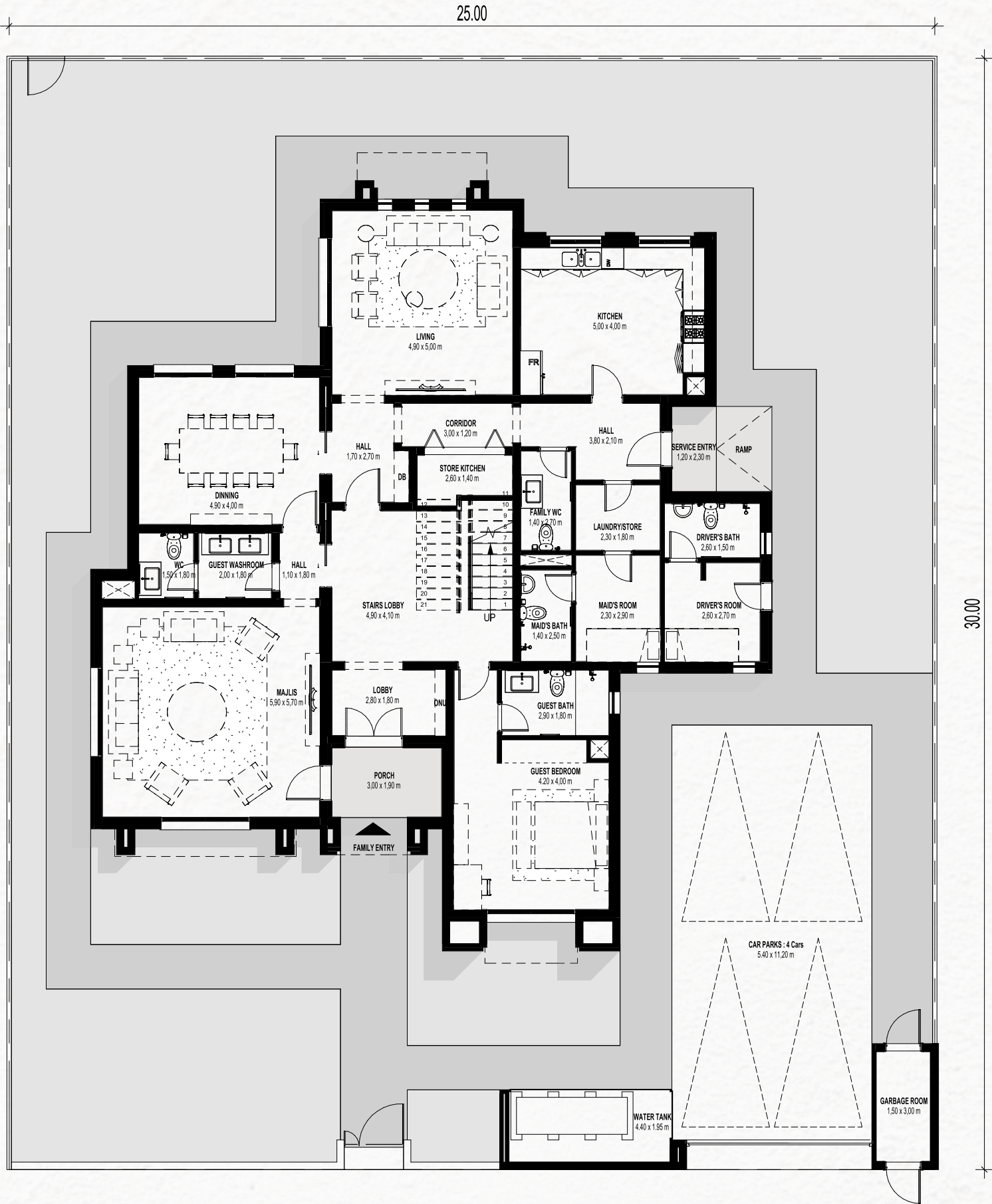
GROUND FLOOR
