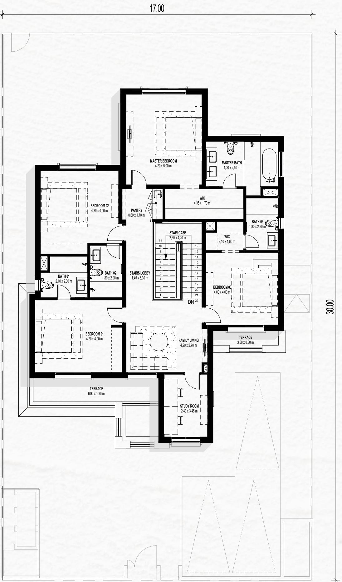
FIRST FLOOR
