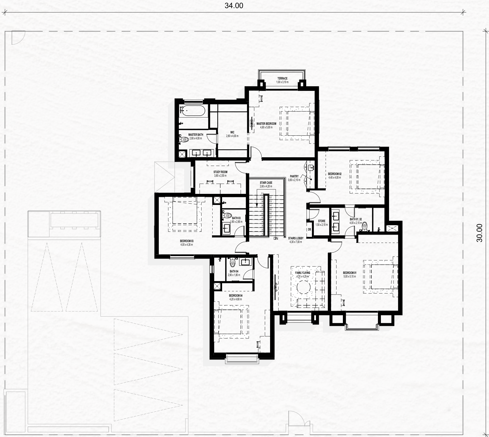
FIRST FLOOR
