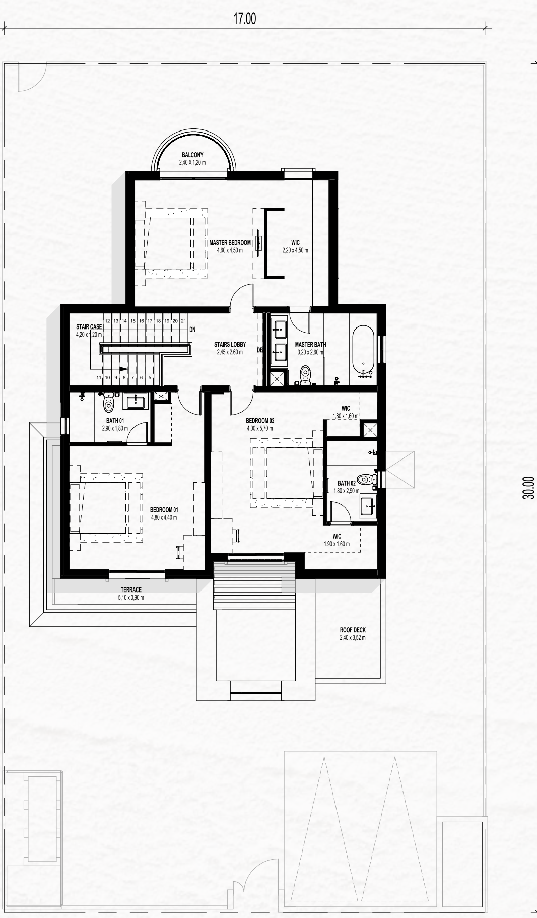
FIRST FLOOR
