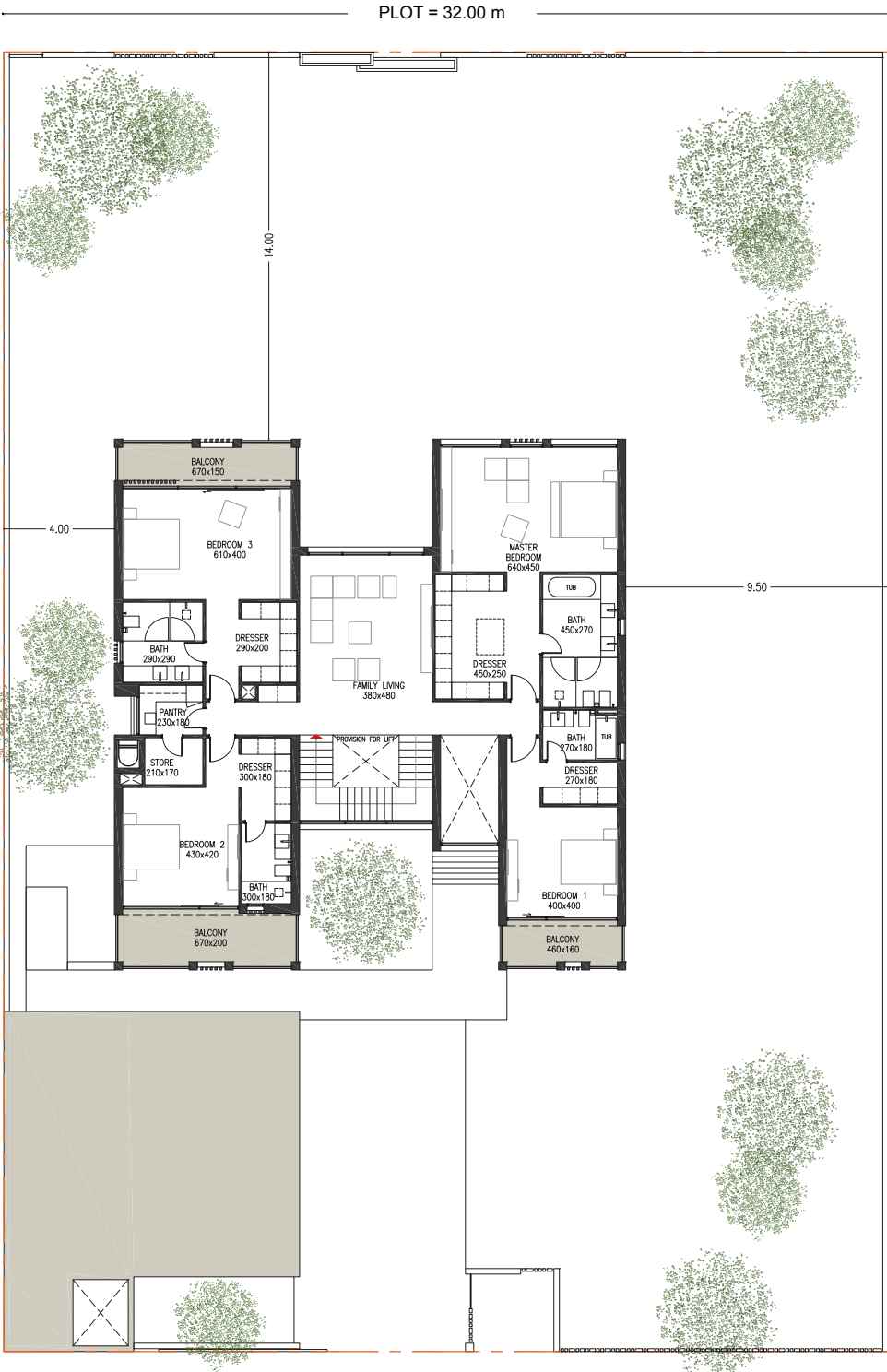
First Floor
