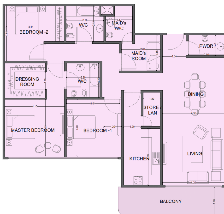
3 BR – SIMPLEX – 1
