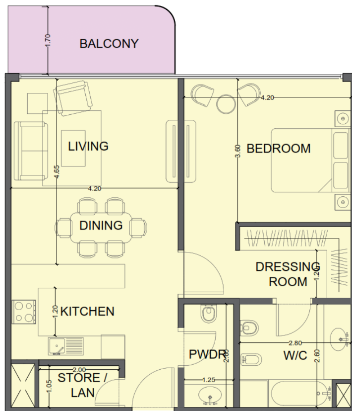
1 BR – SIMPLEX – 1
