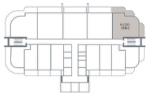
T3 - LEVEL 13 - 29
