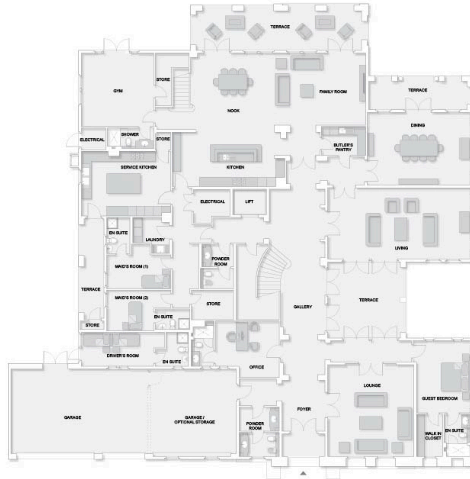
Ground Floor
