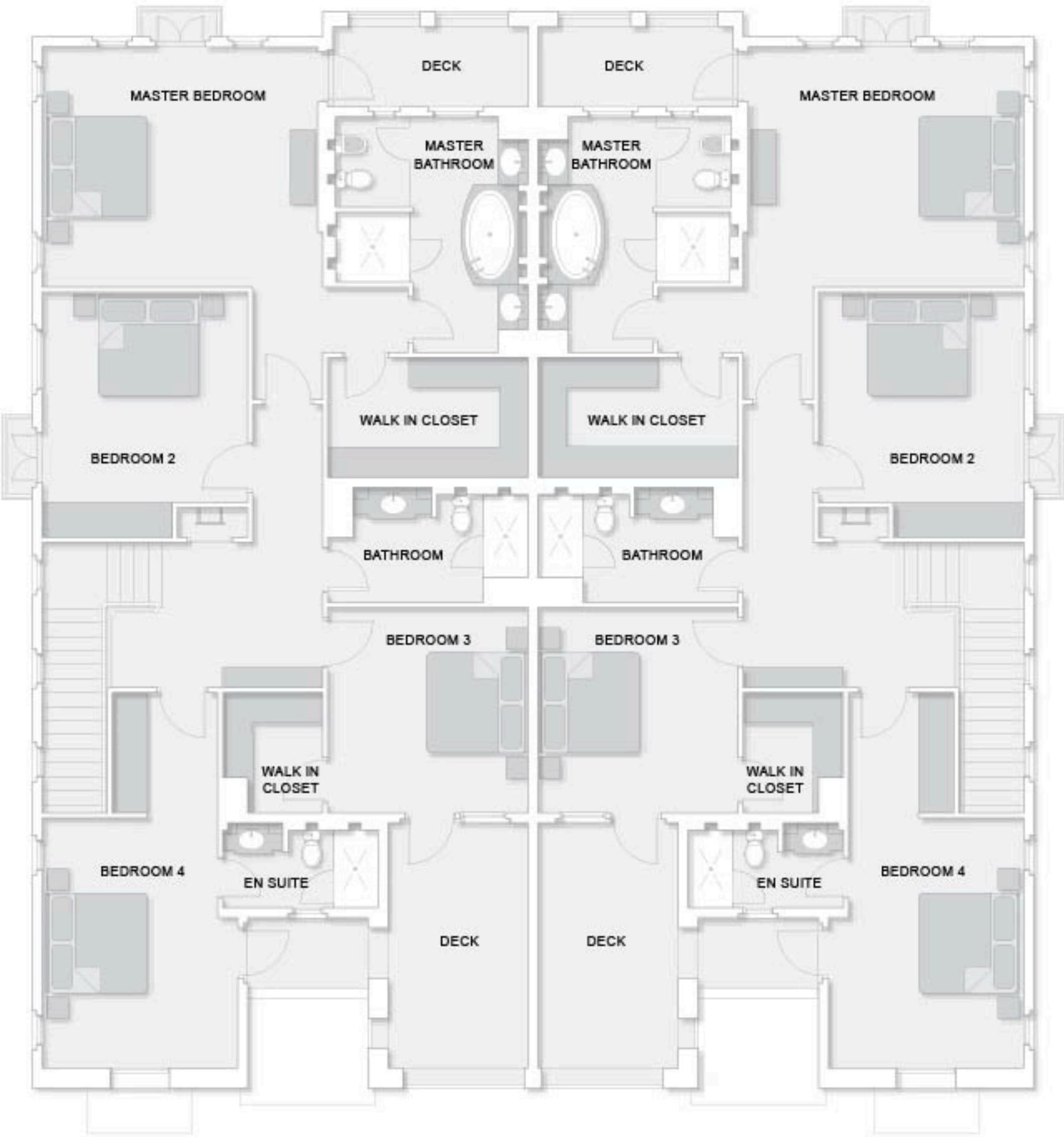
First Floor
