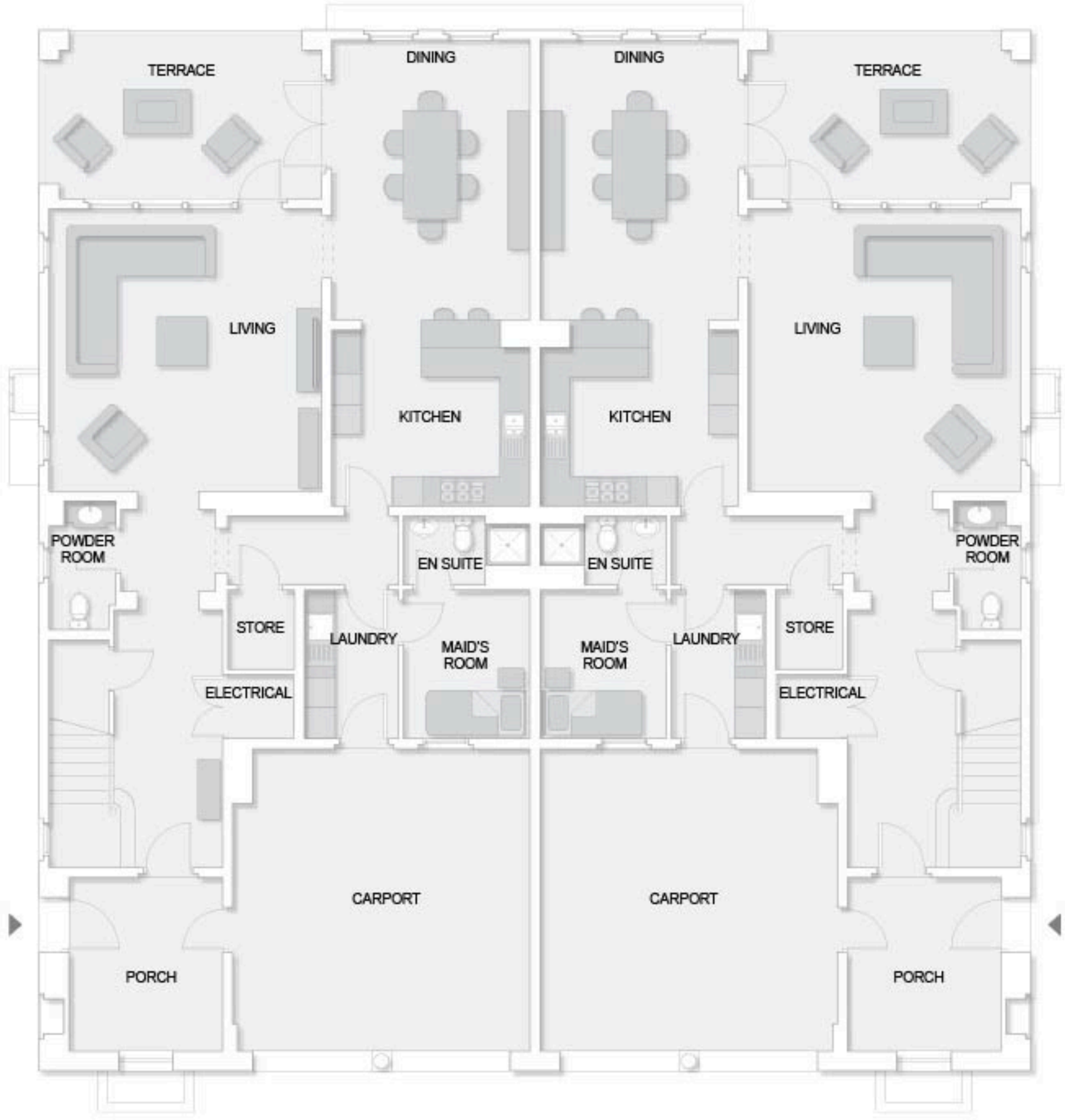
Ground Floor
