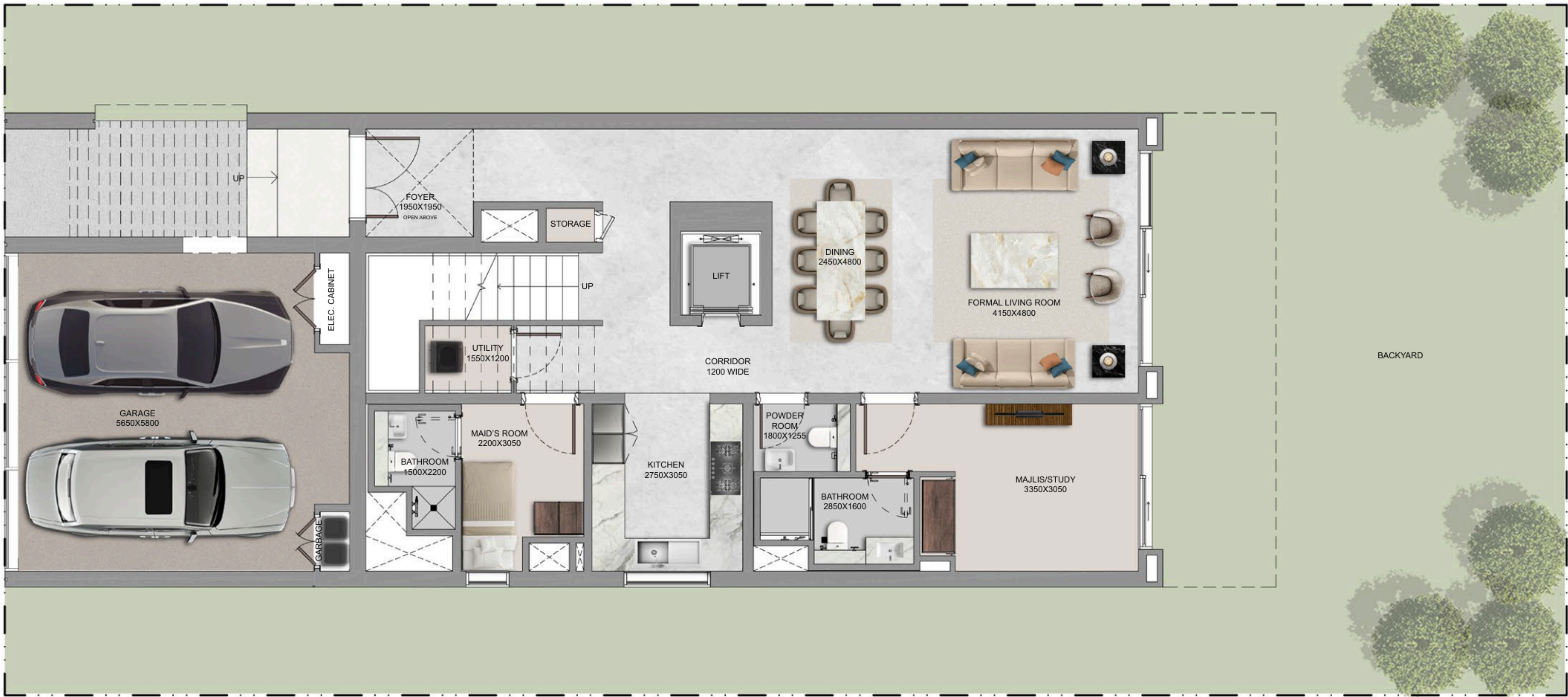
GROUND FLOOR
