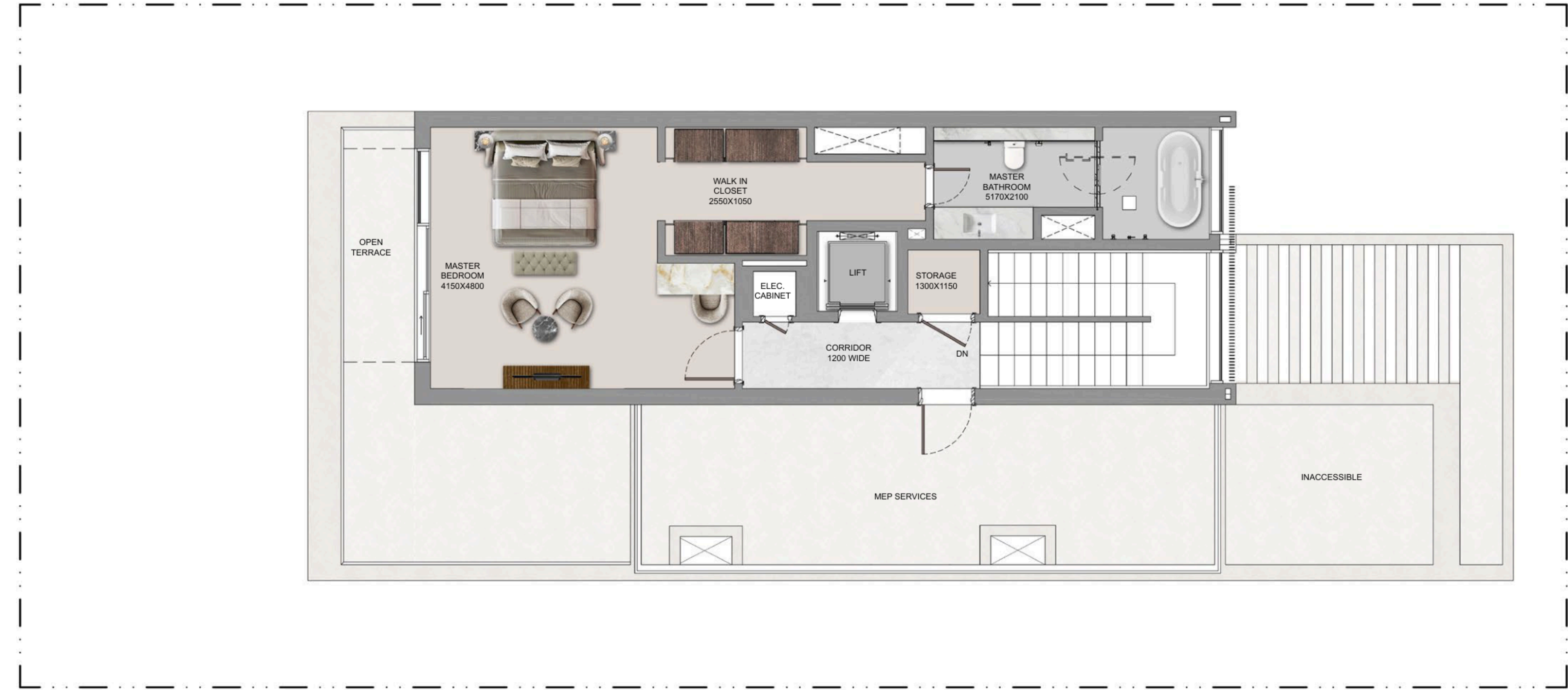
SECOND FLOOR
