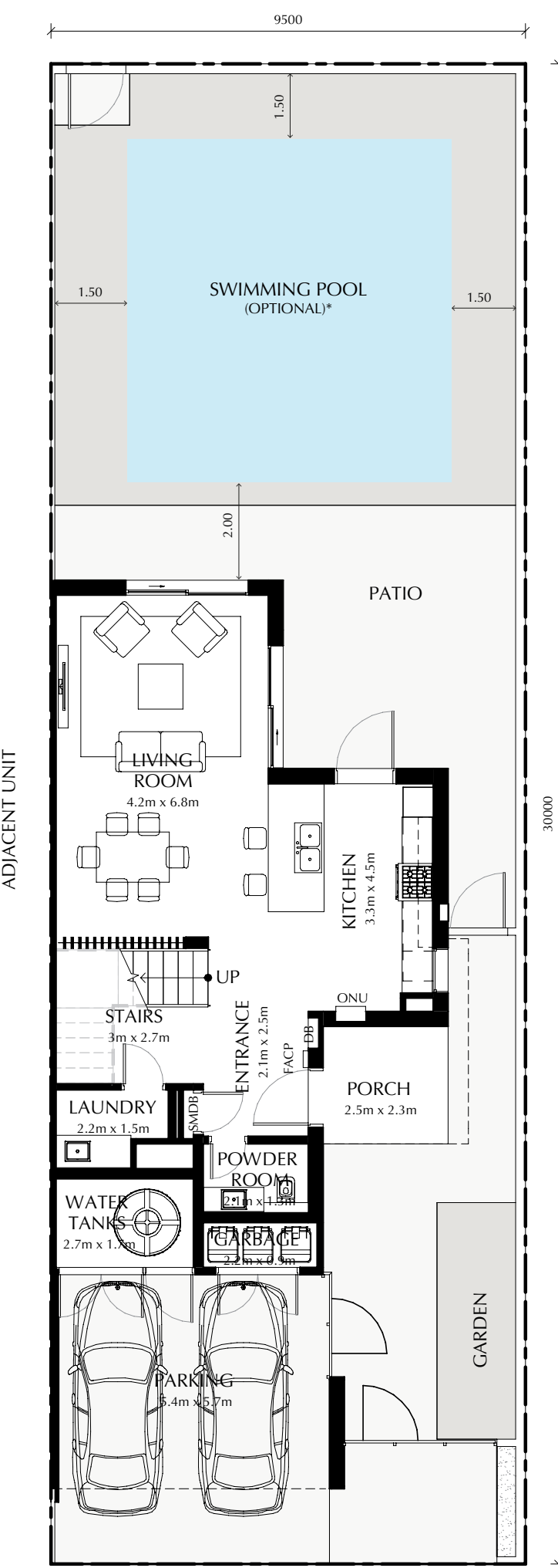
Ground Floor
