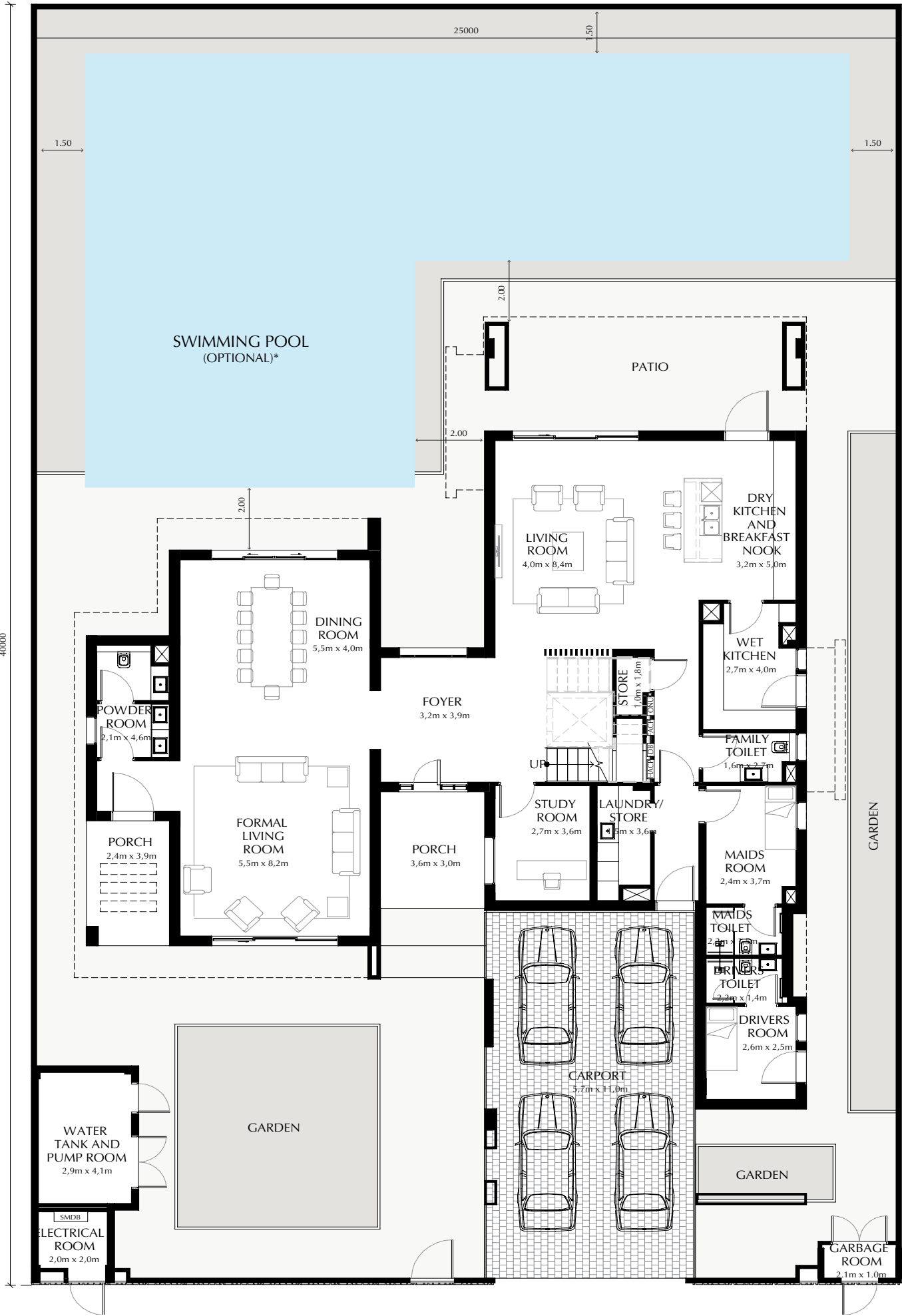
Ground Floor
