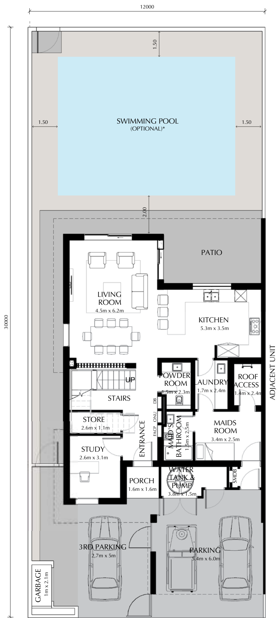
Ground Floor
