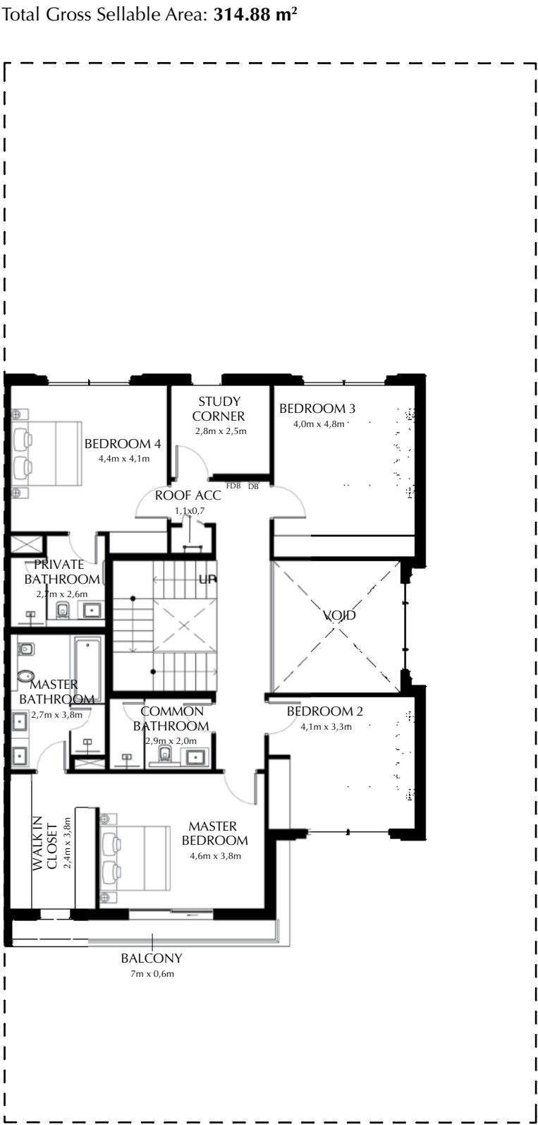
First Floor
