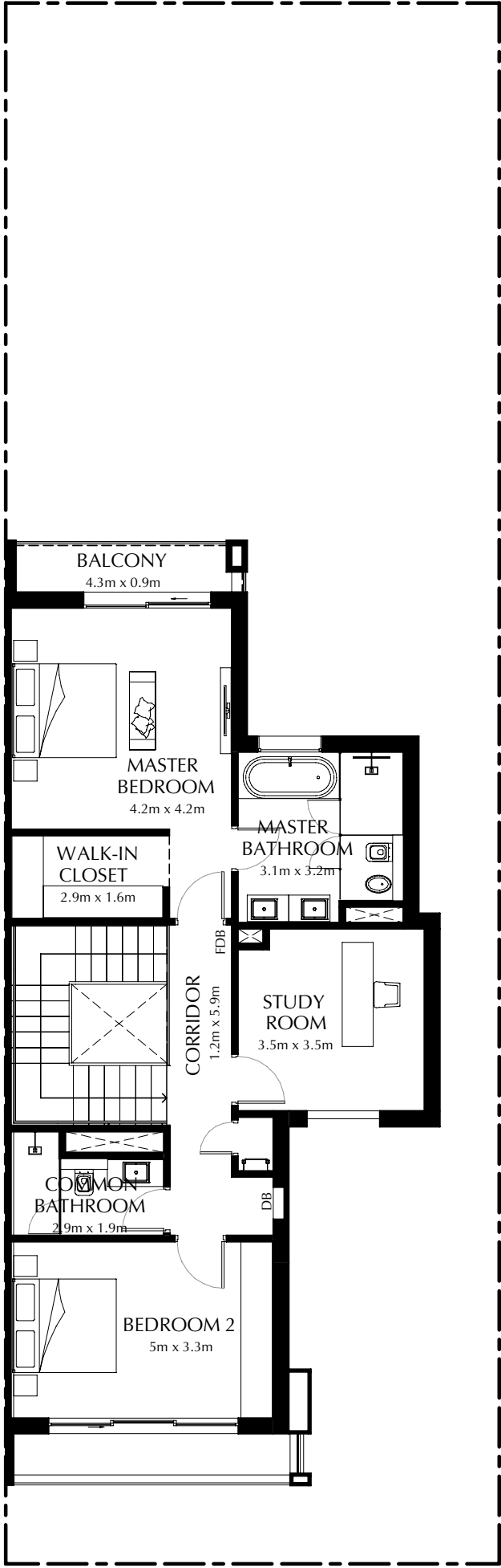
First Floor
